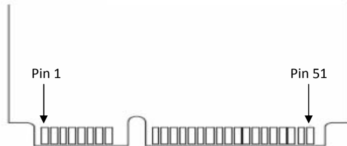
Figure 1-2: Pin assignment
