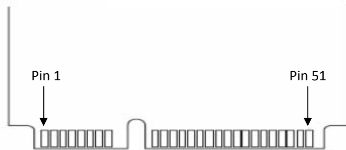
Figure 1-2: mSATA N pin assignment
